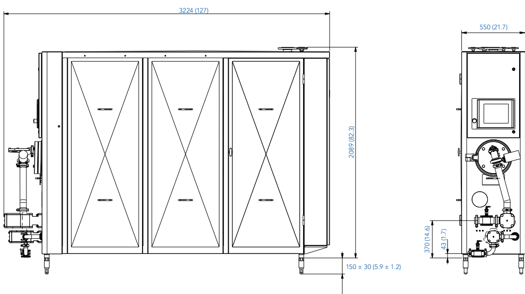
Measurements in mm (inches)
