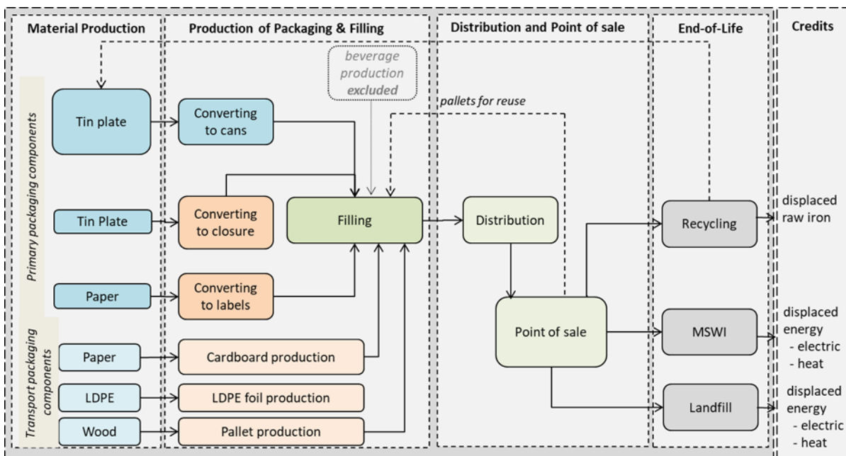
Figure 6: System boundaries steel can
